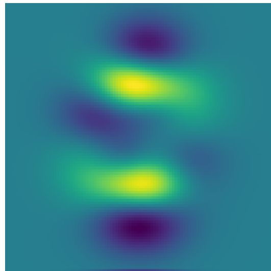
\partial f/\partial x
