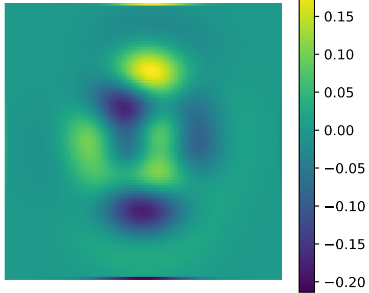
\partial^2 f / \partial x^2 + \partial^2 f / \partial y^2
