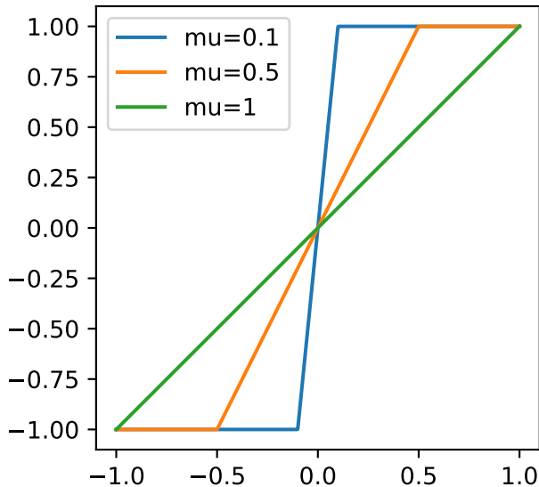
Derivative of Moreau Envelope
