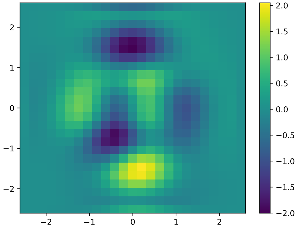
Directional Laplacian
