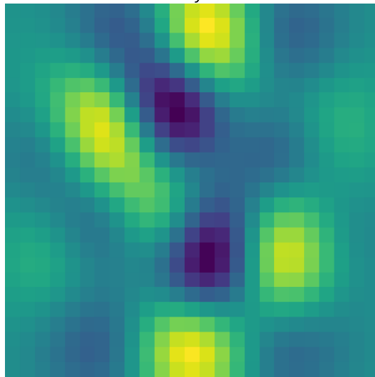
\frac{\partial^3 f(x,y)}{\partial x \partial y^2}
