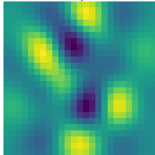
\frac{\partial^3 f(x,y)}{\partial x \partial y^2}
